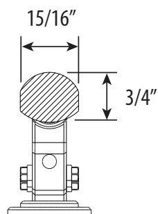
END VIEWS
